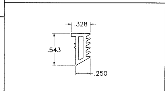
①①A GLAZING WEDGE SCALE 1:1
