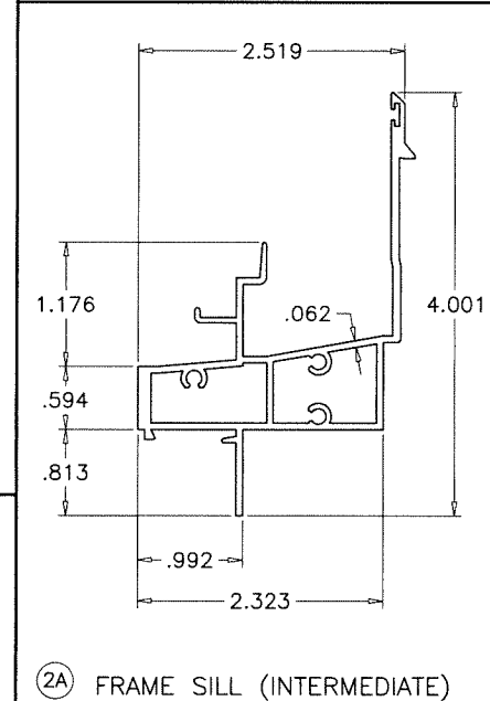
② FRAME SILL
