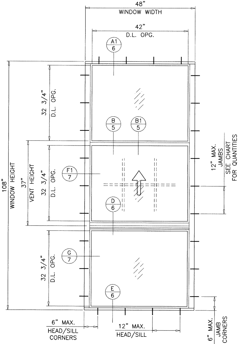
TYPICAL ELEVATION
