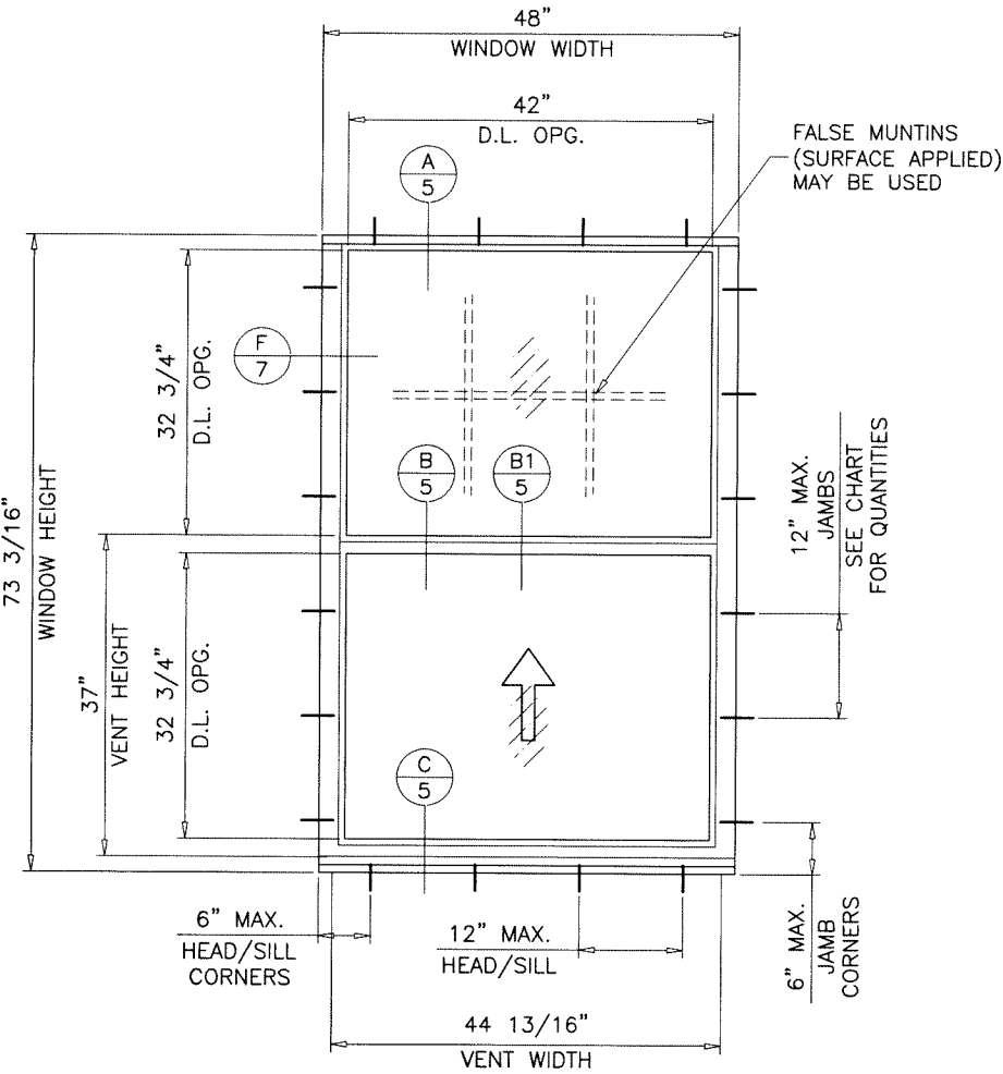
TYPICAL ELEVATION
