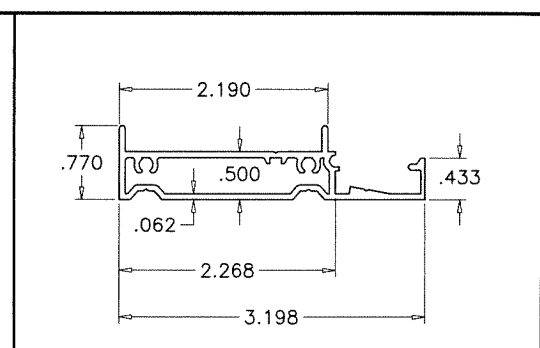
①⑨ FLUSH FRAME ADAPTER
