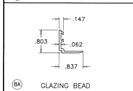
⑧ GLAZING BEAD
