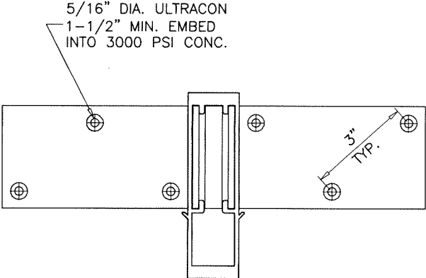
6 ANCHORS @ MULL ENDS
