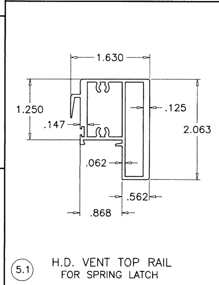
⑤ VENT TOP RAIL FOR SPRING LATCH
